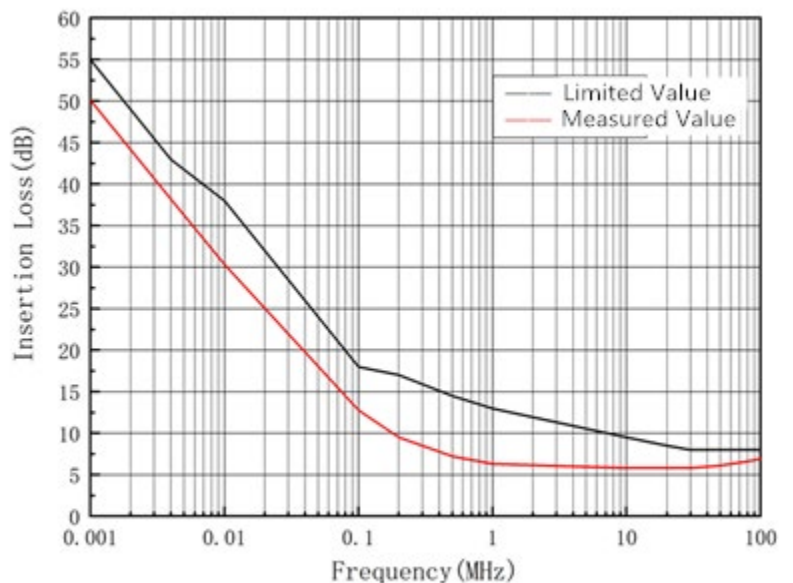
Insertion Loss Curve
