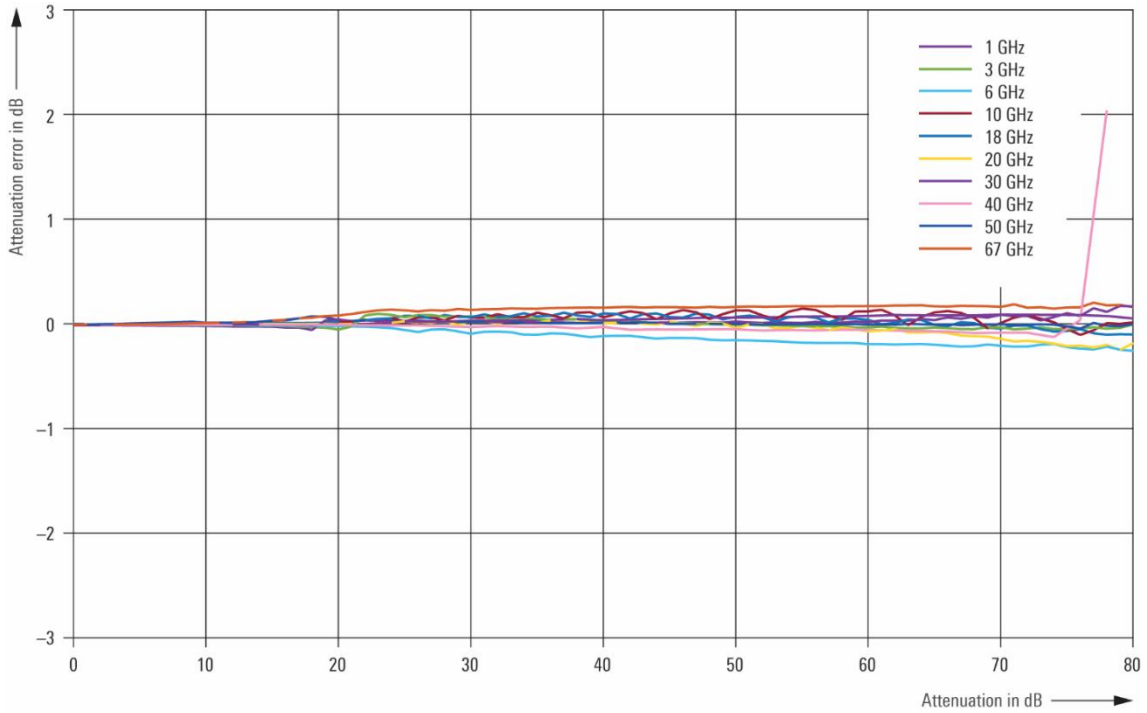
Measured level linearity of high dynamic uninterrupted level sweep with the R&S ® SMAB-K724 option
