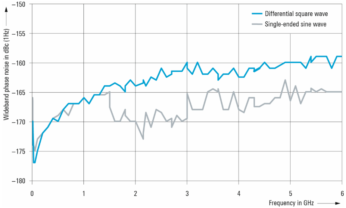
Measured wideband noise of clock synthesizer output at maximum output power versus carrier frequency with the R&S ® SMAB-B29 and R&S ® SMAB-K722 options. Measured with the R&S ® F5WP phase noise analyzer
