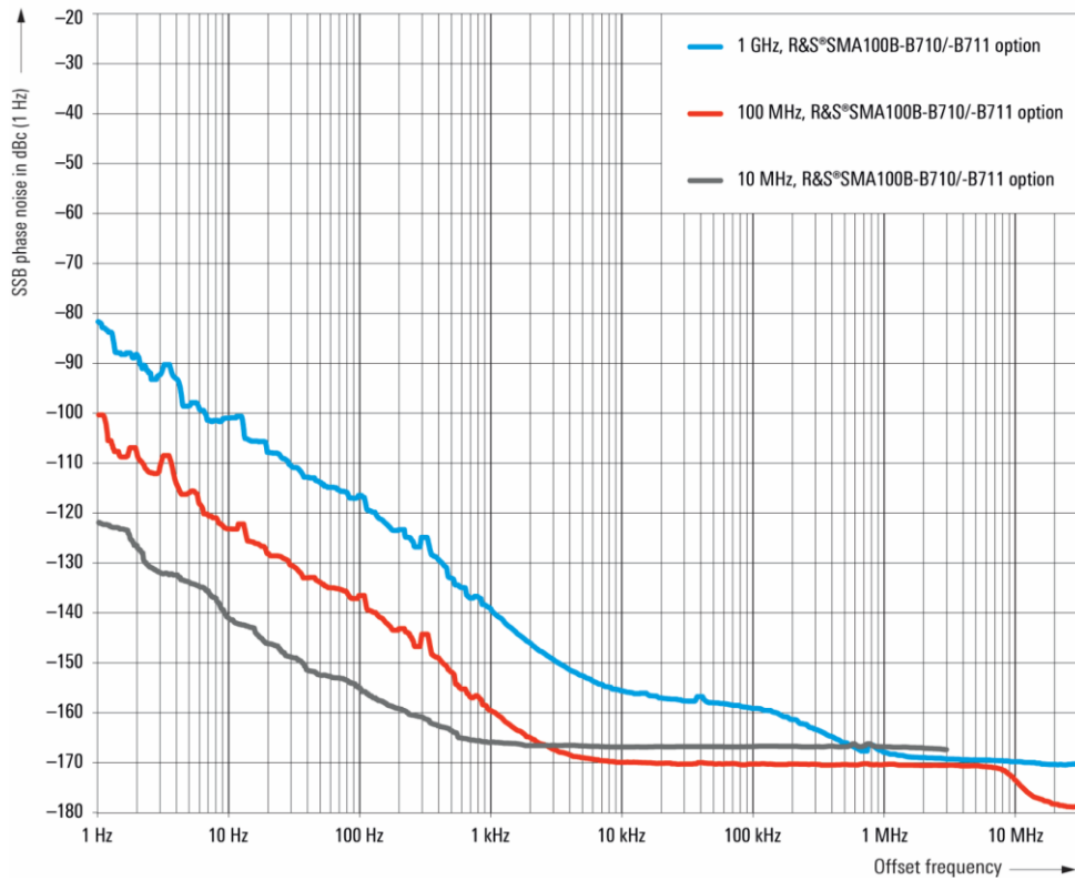
Measured SSB phase noise of reference outputs at f = 10 MHz, 100 MHz and 1 GHz with the R&S ® SMAB-B710(N) and R&S ® SMAB-B711(N) options ( f = 100 MHz and 1 GHz only available with the R&S ® SMAB-K703 option)
