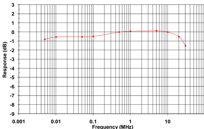
FL7030 Typical Uncalibrated Frequency Response
