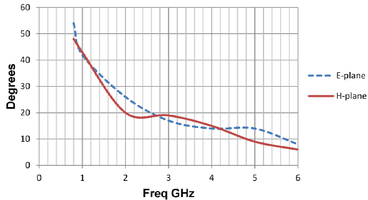
ATH800M6G 3dB Bandwidth
