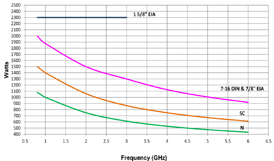
ATH800M6G Input Power
