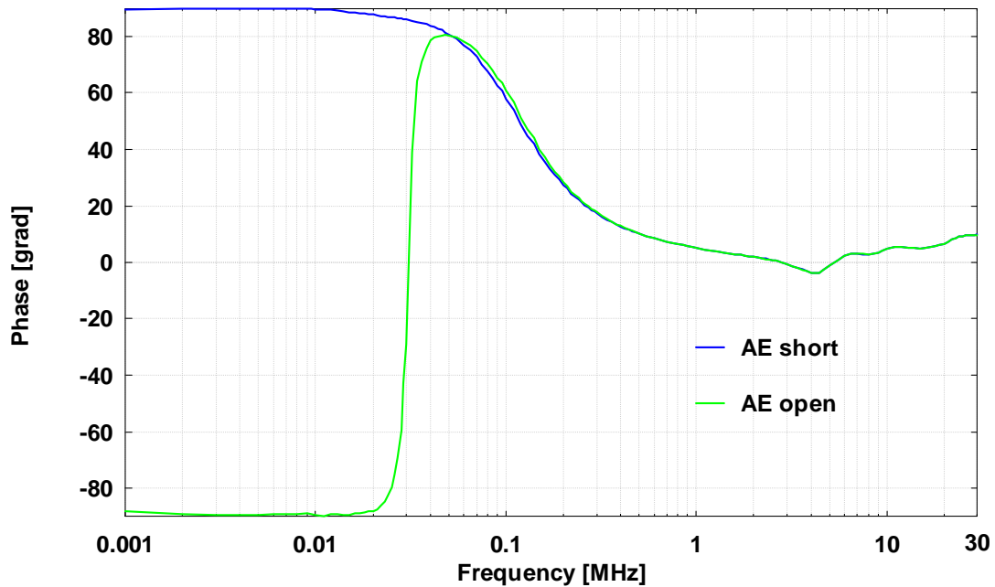
Phase an den Prüflingsklemmen - differential mode, (Kalibrieradapter erforderlich), BNC mit 50 \Omega Abschluss Phase at EuT-Terminals (Calibration adapter required), BNC-Port is terminated with 50 \Omega
