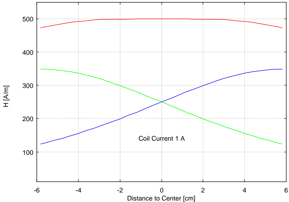
HHS 5202-81 magnetic Fieldstrength along longitudinal coil axis
